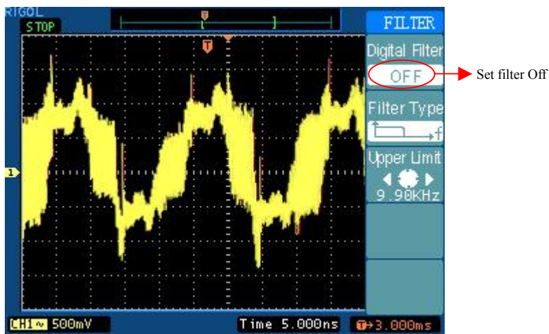
The waveform before filtered
