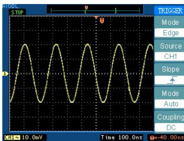
Figure 2-19: Trigger controls
