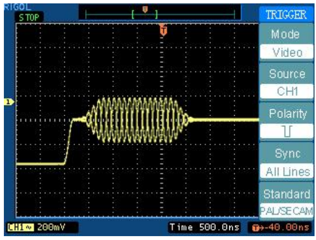
Figure 2-19: Line synchronization
