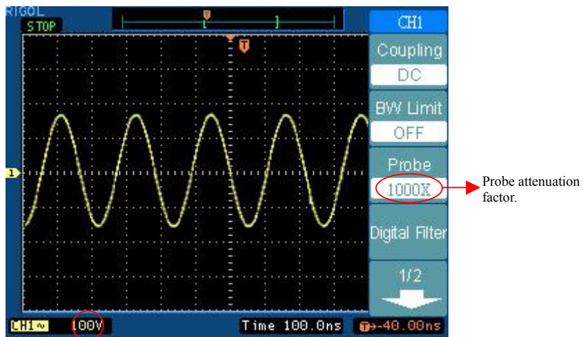
Status changes with the probe attenuation Figure 2-6
